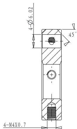
Cross section B-B
