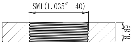
Cross section A-A
