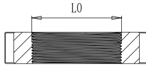
Cross section A-A
