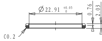
Cross section A-A
