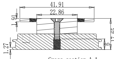
Cross section A-A
